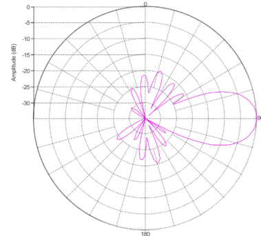
High-Band Vertical pattern (2.2GHz)
