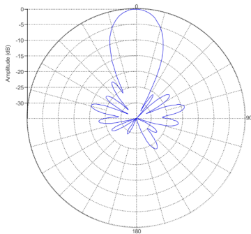
High-Band Horizontal Pattern (2.2GHz)
