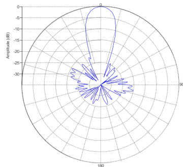
F-Band Horizontal Pattern (3.8GHz)
