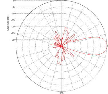
F-Band Vertical pattern (3.8GHz)
