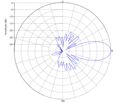
F-Band Vertical pattern (3.8GHz)
