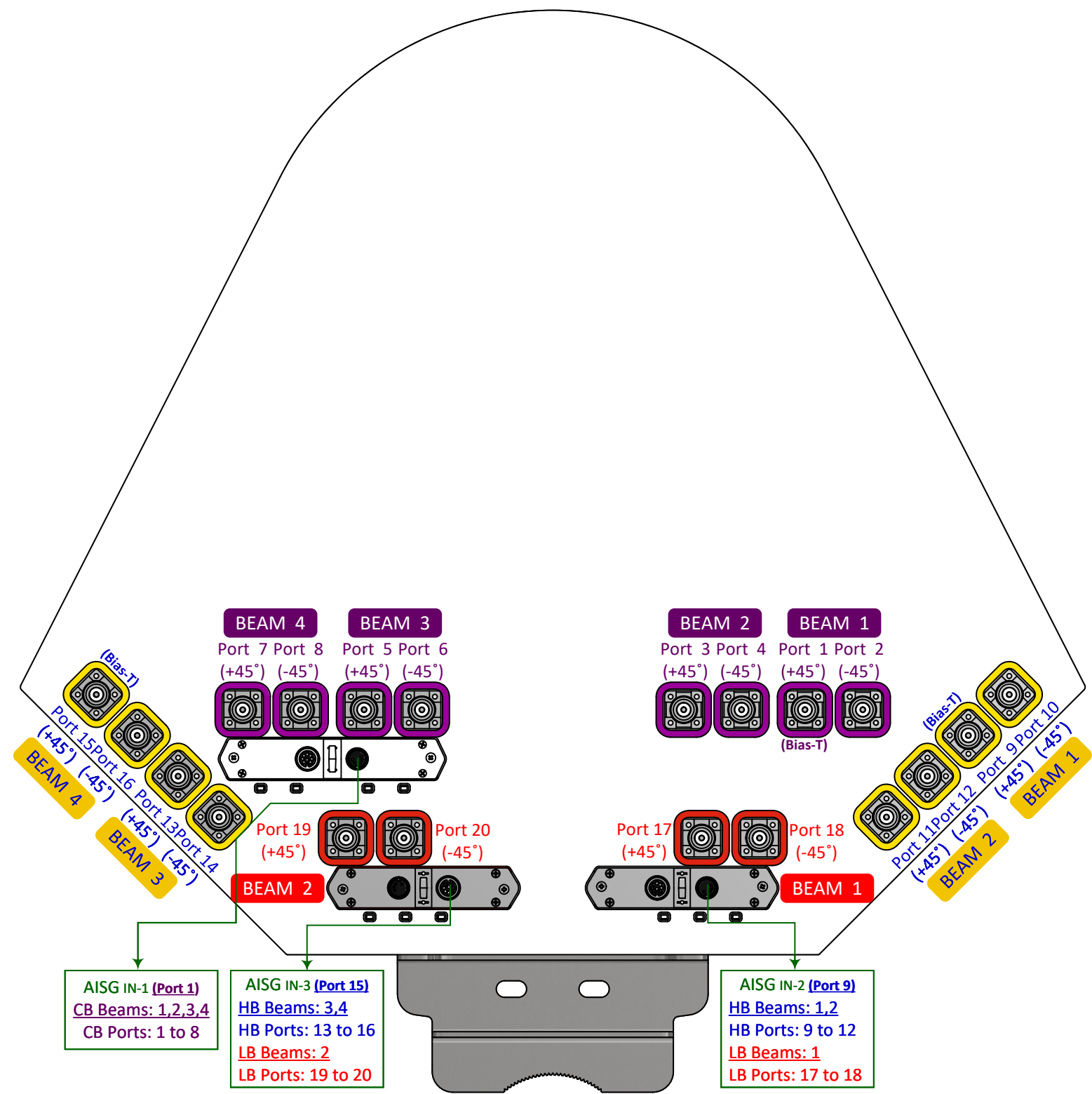
PLAN VIEW CONNECTOR LAYOUT
