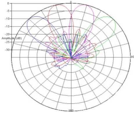
Horizontal Patterns
