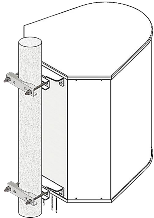
After Installation
