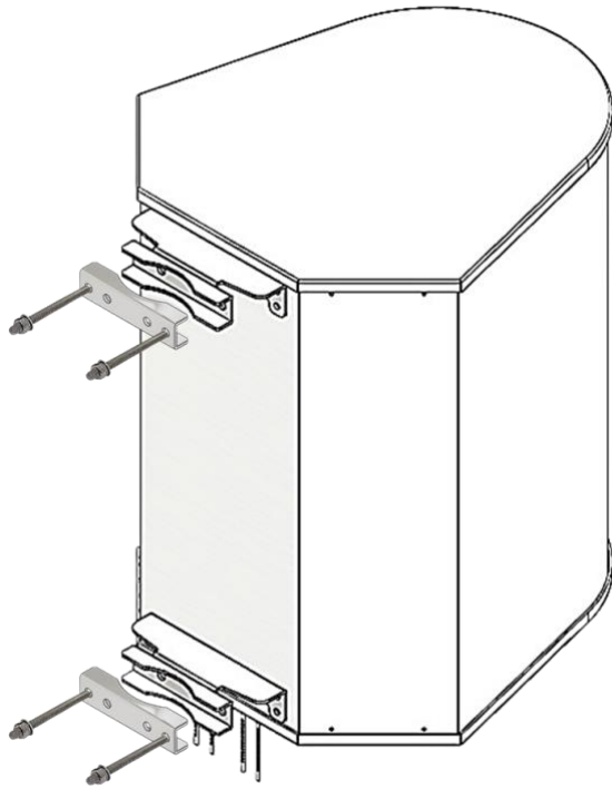
Before Installation
