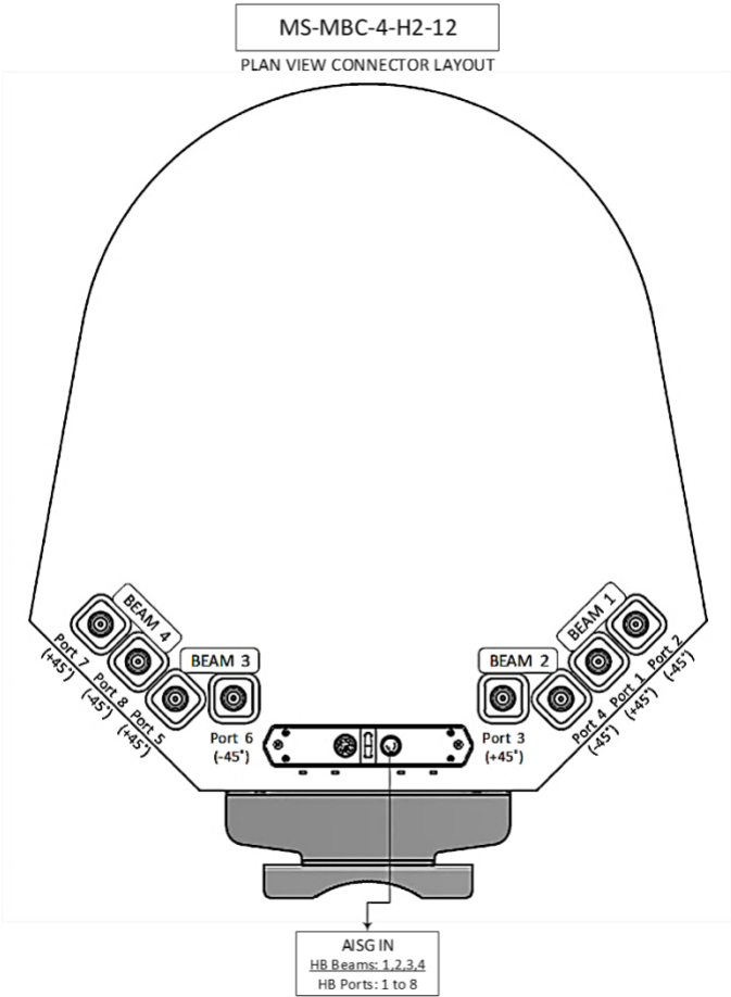
Antenna top view
