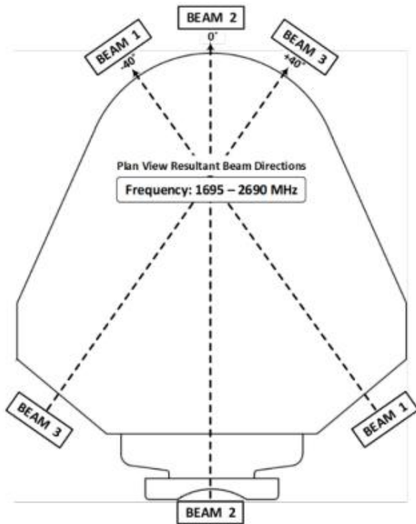
Antenna top view
