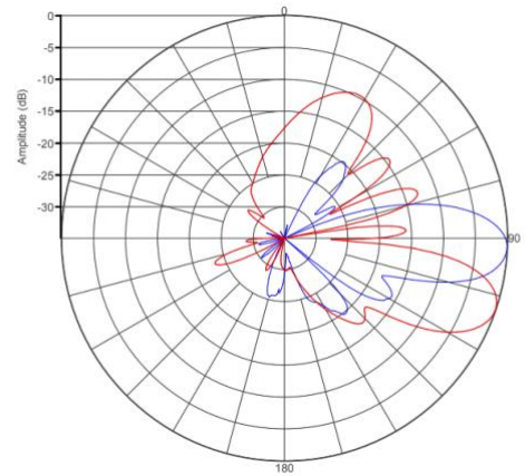
Vertical Patterns (2°, 16°)
