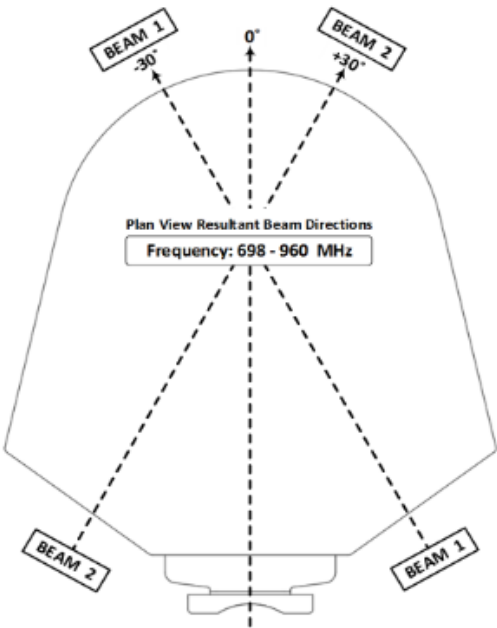
Antenna top view
