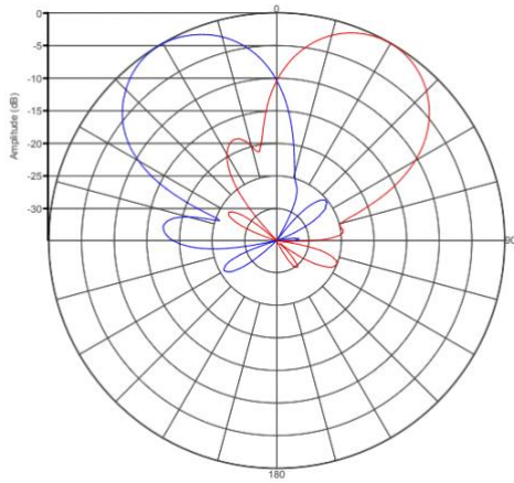
Horizontal Patterns
