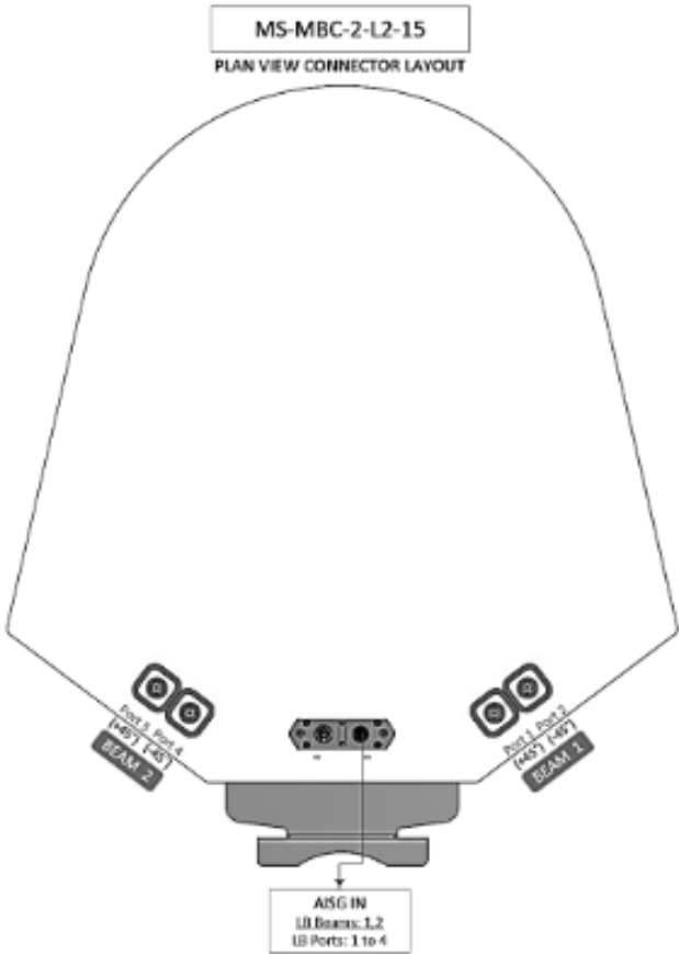
Antenna top view
