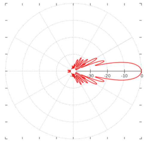
High-band Vertical Pattern (1.92GHz) at tilt 0° and 15°
