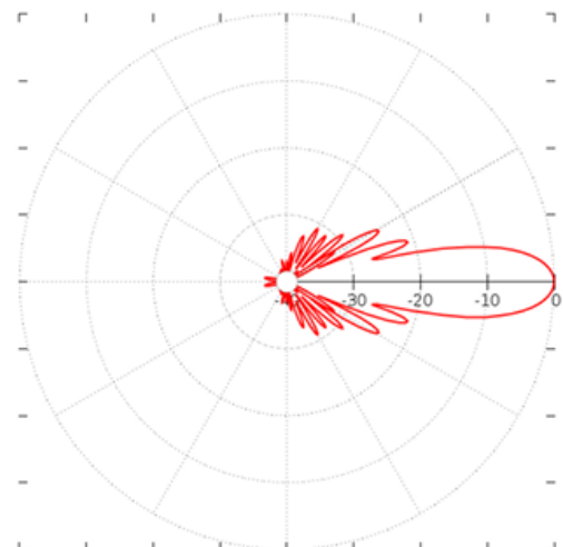
High-band Vertical Pattern (1.92GHz) at tilt 0° and 15°
