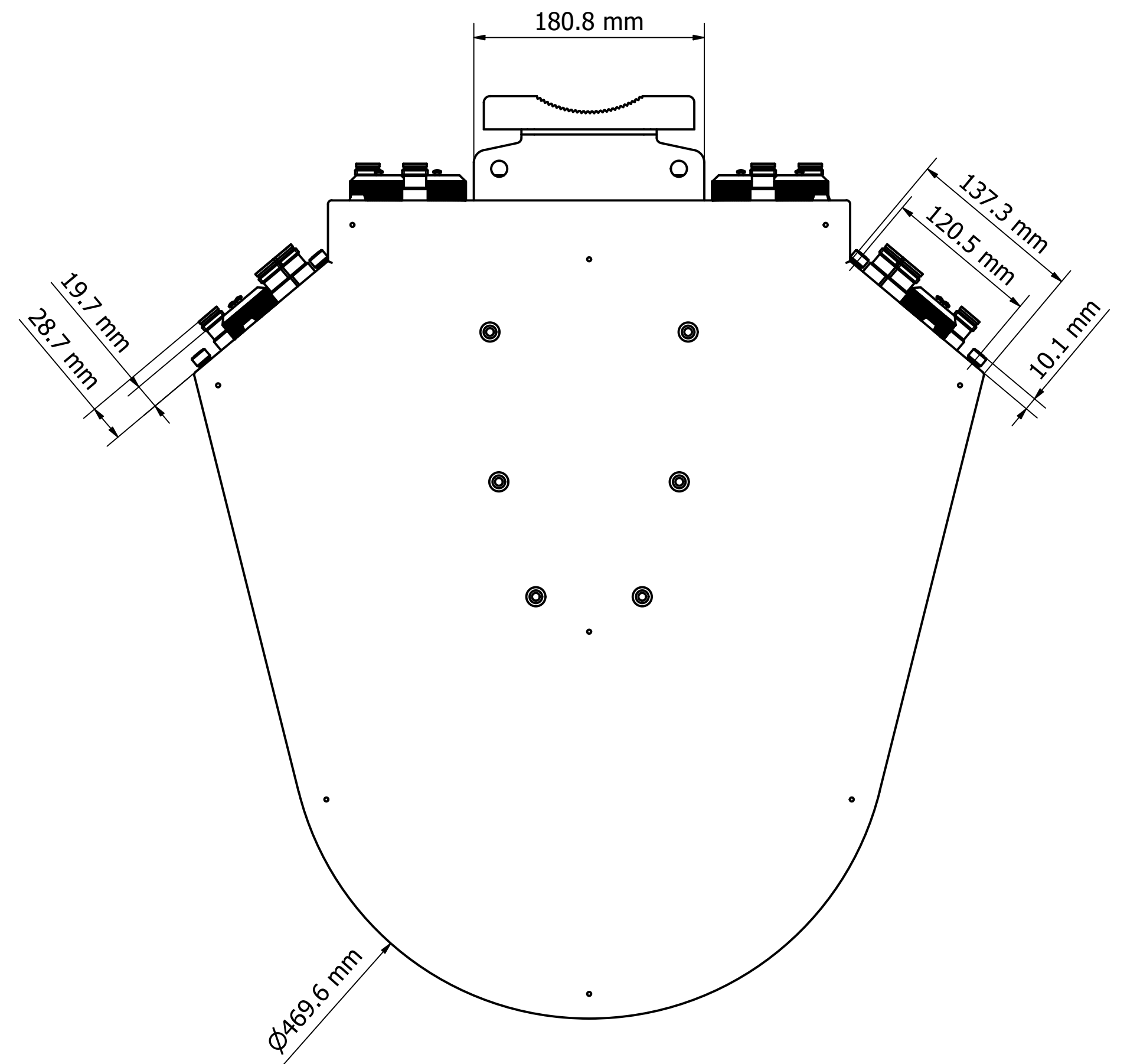
Bottom View
