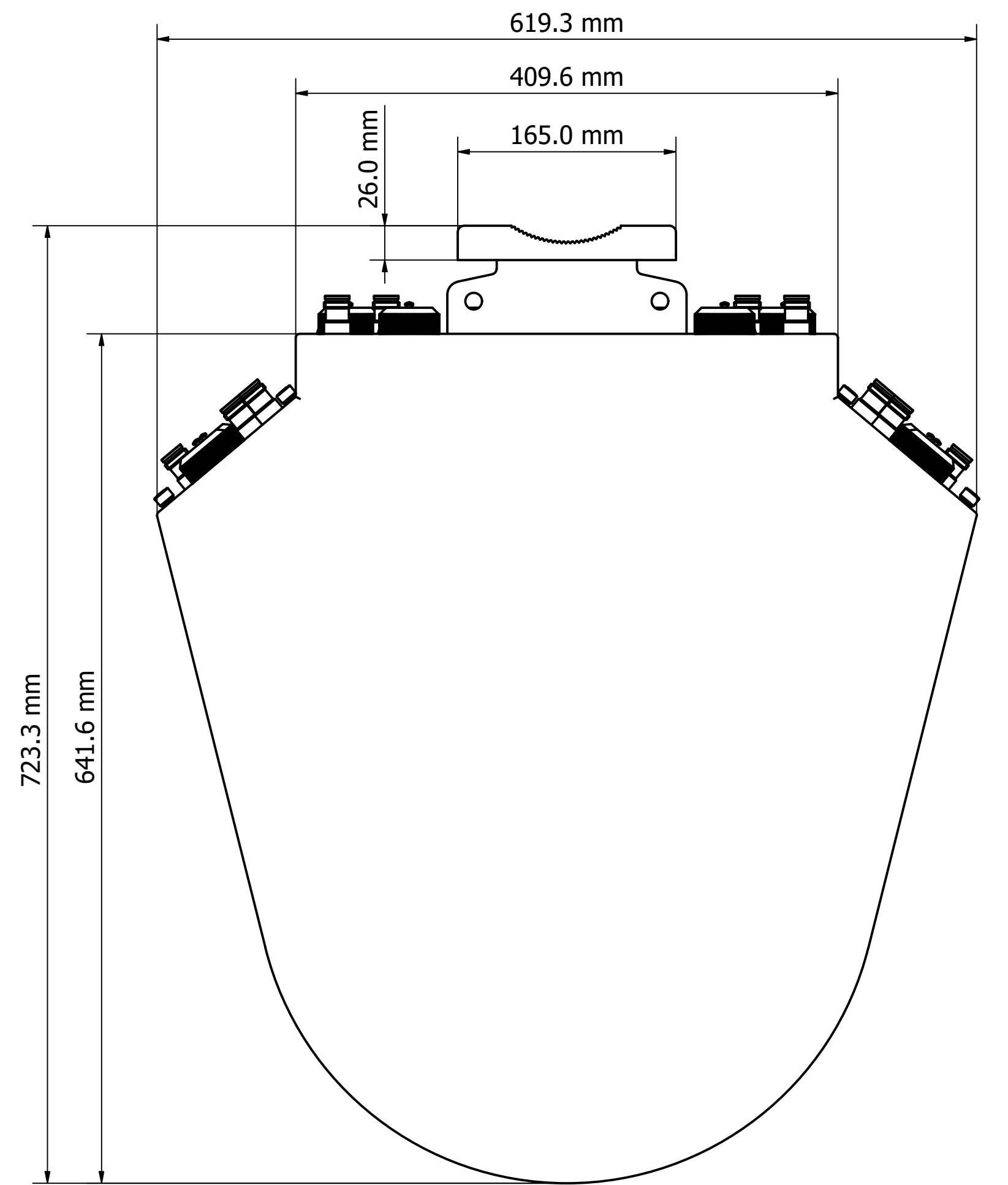
Top View
