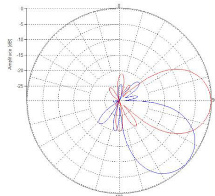
Low-band Vertical Pattern (0.8GHz) at tilt 0° and 40°
