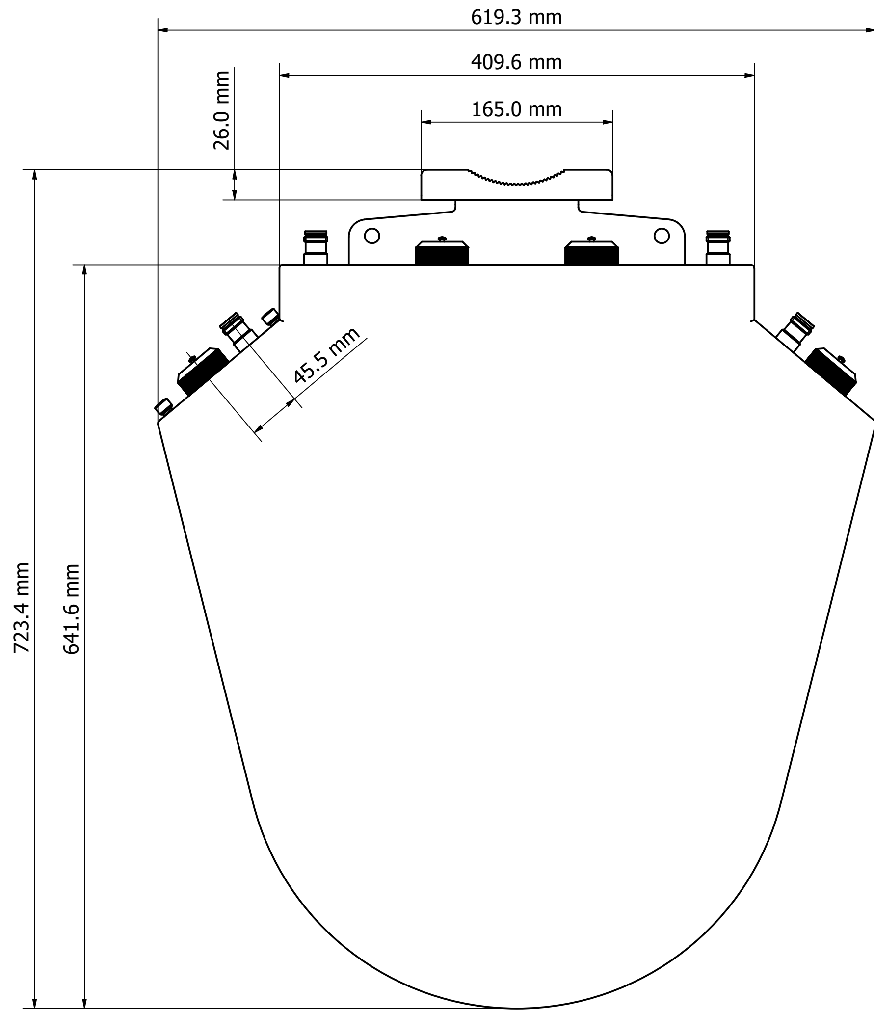
Top View
