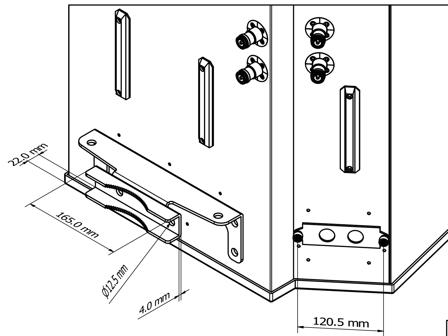
Detail B
