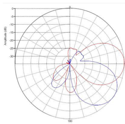
Low-Band Vertical Pattern 0° tilt and 40° tilt (0.8GHz)
