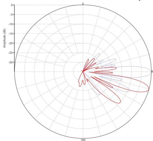
High-Band Vertical Pattern at 0° and 30° Tilt (1.8GHz)
