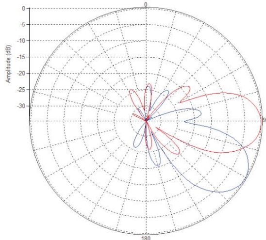
High-Band Vertical Pattern at 0° and 30° Tilt (1.8GHz)
