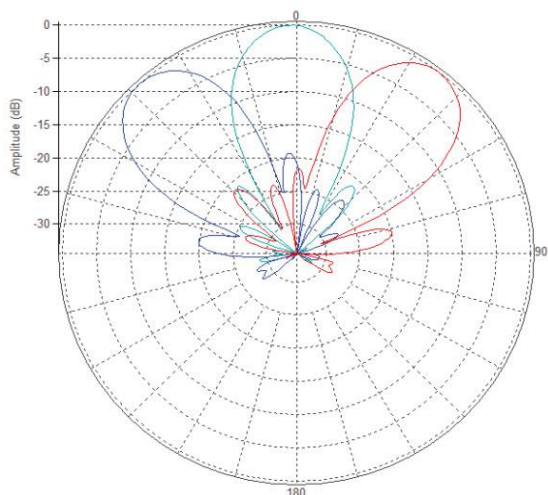
High-Band Horizontal Pattern (1.8GHz)
