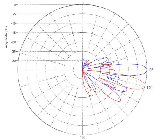
High-Band Vertical Pattern at 0° and 15° Tilt (1.8GHz)
