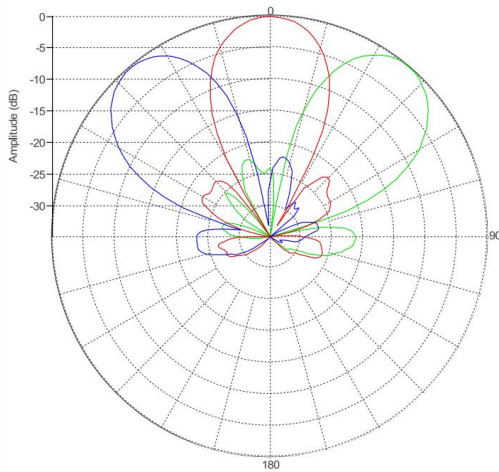
C-Band Horizontal Pattern (3.7GHz)
