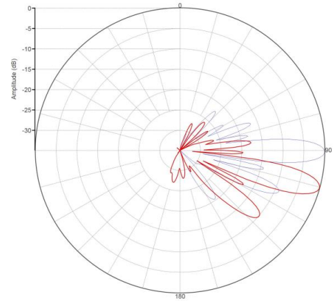
High-Band Vertical Pattern at 0° and 30° Tilt (1.8GHz)
