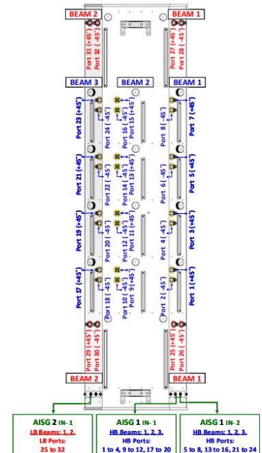
MS-MBA-3.2-H8-L4 (VSON) REAR VIEW CONNECTOR LAYOUT
