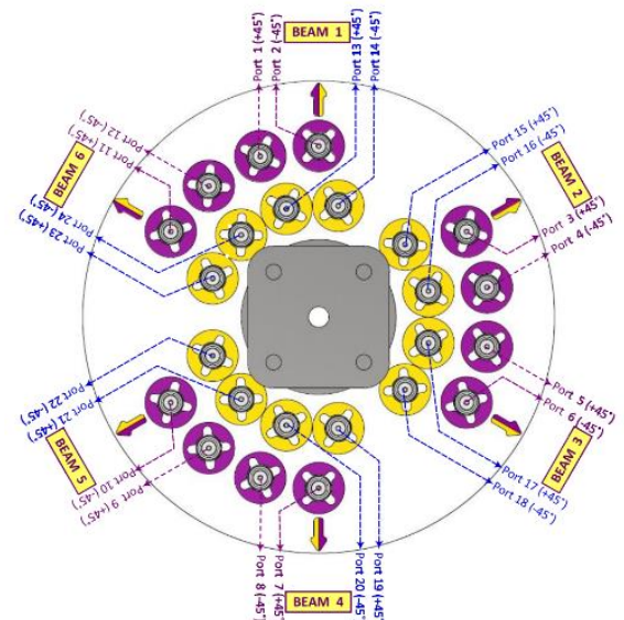
MS-LP-6.6-F2-H2 PLAN VIEW CONNECTOR LAYOUT
