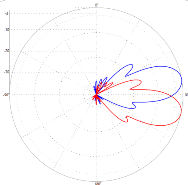
Vertical Pattern (850MHz)
