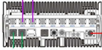
n77 RRU (Samsung RT8808-77A)
