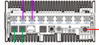
n77 RRU (Samsung RT8808-77A)
