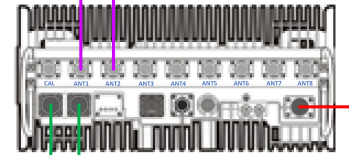
n77 RRU (Samsung RT8808-77A)
