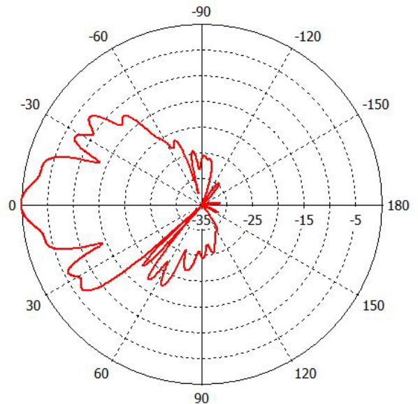
Low-Band Vertical Pattern (700MHz)
