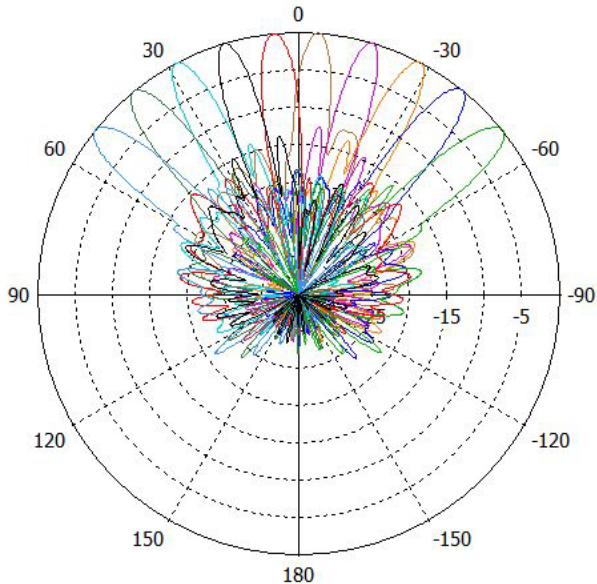
Low-Band Horizontal Pattern (700MHz)
