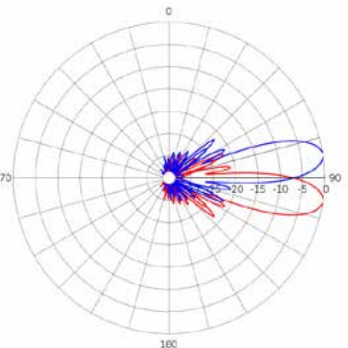
Vertical Pattern
