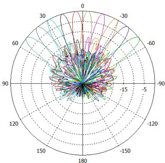
Low-Band Horizontal Pattern (850MHz)
