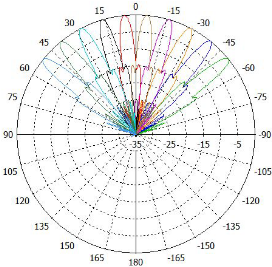
High-Band Horizontal Pattern (1950MHz)
