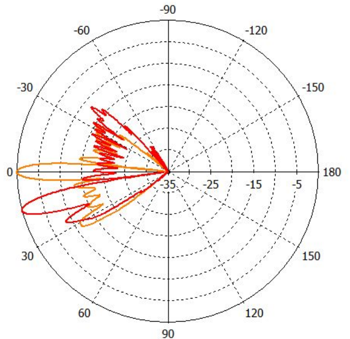
Vertical Pattern 0° tilt
