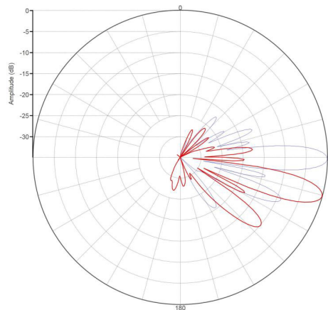
High-Band Vertical Pattern at 0° and 15° Tilt (1.8GHz)
