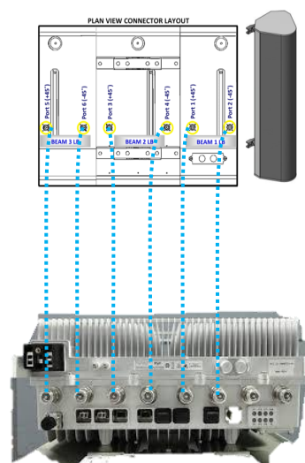
8T8R-RRH-1
