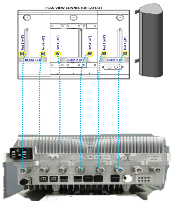
8T8R-RRH-1
