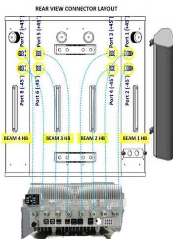
8T8R-RRH-3
