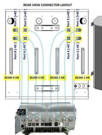
8T8R-RRH-1
