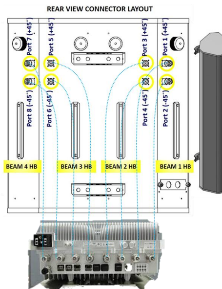
8T8R-RRH-1
