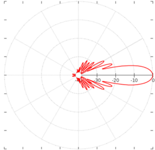
Low-Band Vertical Pattern 0° tilt and 20° tilt (750MHz)
