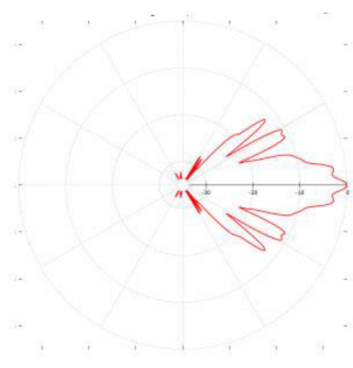
Low-Band Vertical Pattern (700MHz)
