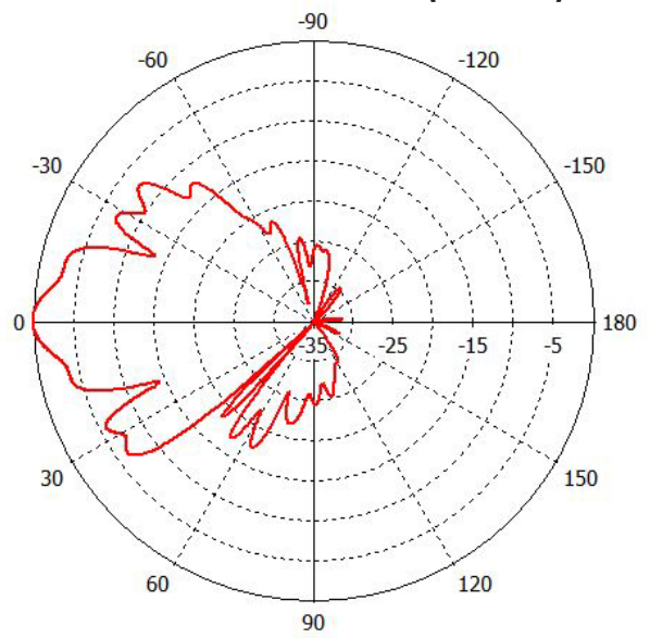
Low-Band Vertical Pattern (700MHz)
