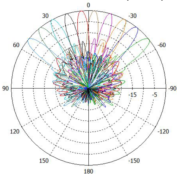
Low-Band Horizontal Pattern (700MHz)
